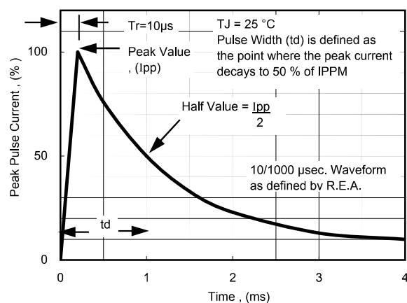
Fig. 5 - Pulse Waveform
