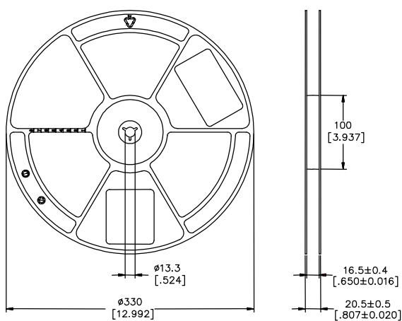
300PCS / Reel
